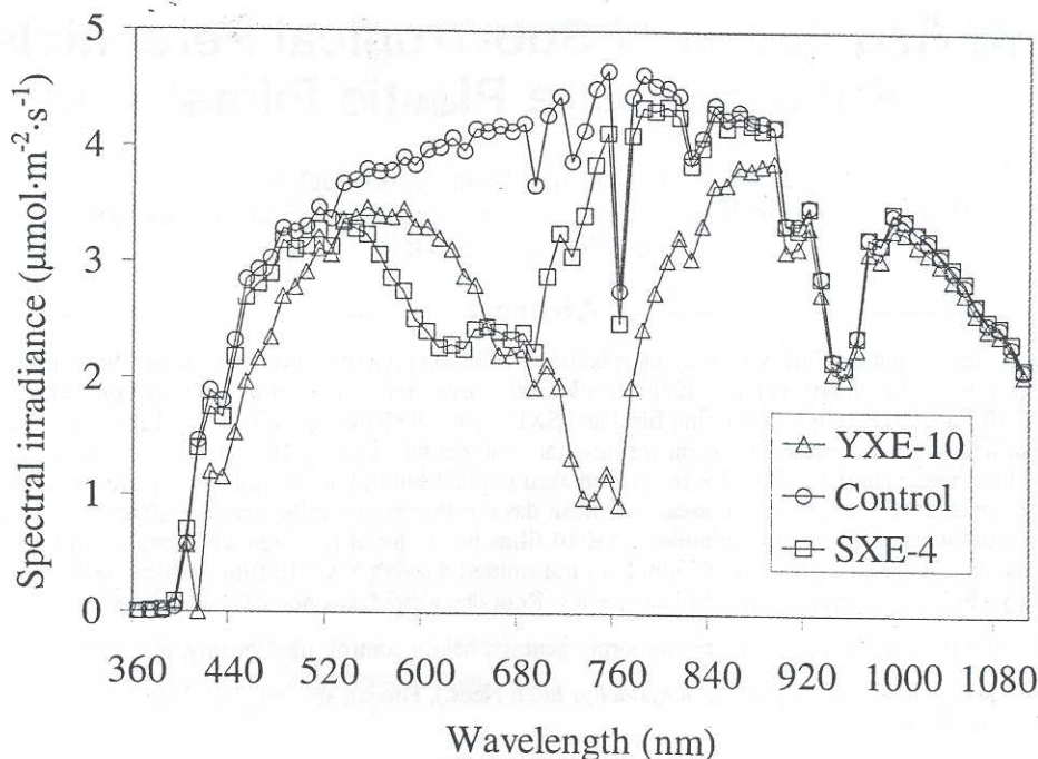
Fig. 1. Spectral transmission properties of YXE-10 (far-red light absorbing) and SXE-4 (red light absorbing) photosensitive films. Control film is a polyethylene film without dye.
